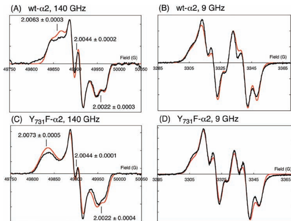
Figure 6. EPR spectra at 140 and 9 GHz of pathway Y^{\bullet} radicals observed in the wt- \alpha 2 and Y_{731}F - \alpha 2 reactions. The reactions were carried out at room temperature with 170 \mu M wt- or Y_{731}F - \alpha 2 , 170 \mu M [NO_2Y_{122}^{\bullet}]\text{-}\beta 2 , 3 mM ATP, and 1 mM CDP and freeze-quenched in the cryostat after \sim 15 s. The 140 and 9 GHz spectra for each reaction were simulated (red traces) using the same set of parameters (Table 1) as described in the text. The g values determined by the simulation are indicated in (A) and (C).
