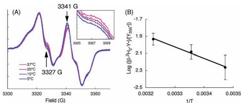
Figure 10. (A) Overlaid EPR spectra of the [\text{NO}_2\text{Y}_{122}\cdot]\text{-}\beta_2/[\beta\text{-}^2\text{H}_2]\text{Y-}\alpha_2/\text{ATP/CDP} reaction at 5 (blue), 15, 25, and 37 °C (red) without subtraction of the \text{NO}_2\text{Y}^\bullet spectrum. The arrows indicate the change induced by the shift in the temperature. Each spectrum is an average of two or three experiments. The inset is a magnified view between 3325 and 3330 G. (B) \log([\beta\text{-}^2\text{H}_2]\text{Y}^\bullet/[\text{Y}_{356}\cdot]) vs 1/T . The [\beta\text{-}^2\text{H}_2]\text{Y}^\bullet values determined for the reactions at 15, 25, and 37 °C were used. At 5 °C, the amount of [\beta\text{-}^2\text{H}_2]\text{Y}^\bullet could not be quantitated. The line is a linear least-squares fit to eq 1 with \Delta E^\circ = 110 mV. Each point represents an average of two or three experiments.
