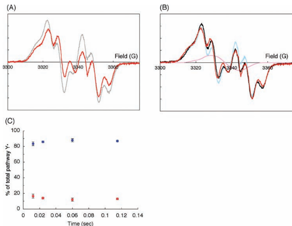
Figure 9. (A) EPR spectrum of pathway Y• radicals observed in the reaction with [\text{NO}_2\text{Y}_{122}^\bullet]\text{-}\beta 2/[\beta\text{-}^2\text{H}_2]\text{Y-}\alpha 2/\text{ATP}/\text{CDP} carried out at 25 °C and quenched at 115 ms (red trace). The EPR spectrum observed in the same reaction using nonlabeled \alpha 2 is overlaid (gray trace). The \text{NO}_2\text{Y}_{122}^\bullet spectrum (50% of the total radical) was subtracted from the observed spectra in both cases. (B) EPR spectral reconstruction using the spectrum of \text{Y}_{356}^\bullet observed in the [\text{NO}_2\text{Y}_{122}^\bullet]\text{-}\beta 2/[\text{Y}_{731}\text{F}]\text{-}\alpha 2/\text{ATP}/\text{CDP} reaction (blue, 87%) and that of [\beta\text{-}^2\text{H}_2]\text{Y}^\bullet simulated using the parameters shown in Table 1 as described in the text (pink, 13%). The sum of the two spectra is shown in the black trace and overlaid with the EPR spectrum of pathway Y• radicals observed in the [\text{NO}_2\text{Y}_{122}^\bullet]\text{-}\beta 2/[\beta\text{-}^2\text{H}_2]\text{Y-}\alpha 2/\text{ATP}/\text{CDP} reaction freeze-quenched at 115 ms (red trace). (C) Time course of the relative ratios of \text{Y}_{356}^\bullet (blue) and [\beta\text{-}^2\text{H}_2]\text{Y}^\bullet (red) at 25 °C determined as described in (B). Each point represents an average of two or three experiments.
