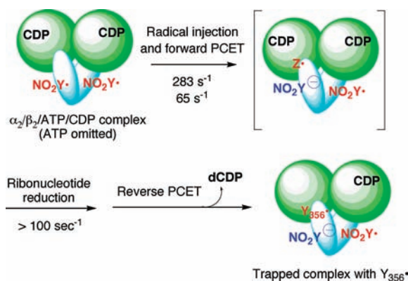
Figure 2. Model for the reaction of [NO 2 Y 122 *]- \beta 2 with \alpha 2, ATP, and CDP based on rapid kinetics experiments. Reprinted from ref 5. Copyright 2010 American Chemical Society. The green circles represent \alpha and the blue ovals \beta . ATP, the allosteric effector, is omitted from \alpha for clarity. There are 1.2 NO 2 Y* radicals/ \beta 2, not 2, as shown in the figure, and their distribution between the two monomers of \beta is not understood. Any intermediate(s) between the forward PCET and ribonucleotide reduction is (are) designated as Z*. Rate constants determined for dCDP and Y* formation ( >100 s -1 ) are limited by the time resolution of the instrument measurement, and these steps likely exhibit biphasic kinetics with rate constants similar to that of the NO 2 Y phenolate formation.
