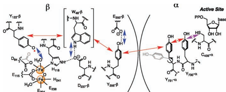
Figure 1. Proposed PCET pathway in E. coli class Ia RNR. Alternative conformations found in crystal structures are shown in gray for D 84 - \beta 2 (PDB ID 1JQC 61 ) and Y 731 - \alpha 2 (PDB ID 2XO4 42 ). Red and blue arrows indicate orthogonal transfer of an electron and proton, respectively. The proton acceptor for Y 731 - \alpha 2 during its transient oxidation is unknown. The purple arrow in \alpha 2 indicates colinear movement of the electron and proton. Y 356 - and E 350 - \beta 2 are in the flexible C-terminal tail and are disordered in all crystal structures. There is currently no direct evidence for the involvement of W 48 - \beta 2 in the radical propagation process, hence indicated by brackets.
