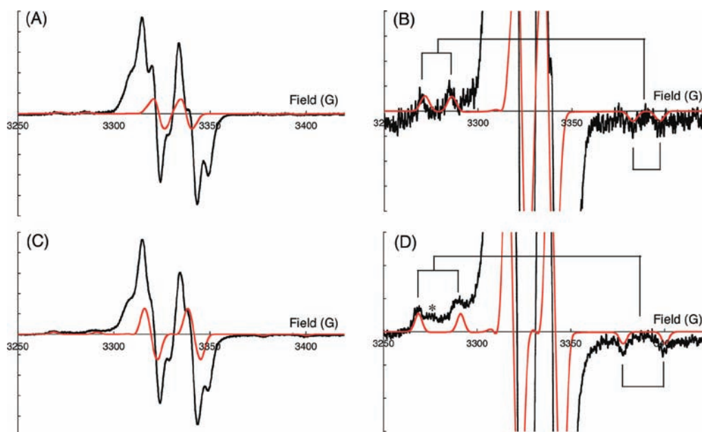
Figure 7. EPR spectra of the pathway radicals formed in the reaction of [3,5\text{-F}_2\text{Y}_{731}]\text{-}\alpha 2 (A, B) or [3,5\text{-F}_2\text{Y}_{730}]\text{-}\alpha 2 (C, D) with [\text{NO}_2\text{Y}_{122}^{\bullet}]\text{-}\beta 2/\text{ATP}/\text{CDP} quenched at 60 ms (black traces) overlaid with simulated EPR spectra of 3,5\text{-F}_2\text{Y}^{\bullet} (red traces). The EPR spectrum of \text{NO}_2\text{Y}^{\bullet} (50% of the total radical) was subtracted from the observed spectrum. (B) and (D) are magnified views of (A) and (C), respectively. The EPR spectral simulations were carried out using the parameters shown in Table 1. Only the low- and high-field doublet features were simulated as described in the text. The asterisk in (D) indicates an uncharacterized signal that has also been observed in the reaction with wt- \alpha 2 . Brackets in (B) and (D) indicate the hyperfine splitting associated with ^{19}\text{F} and \beta\text{-}^1\text{H} .
